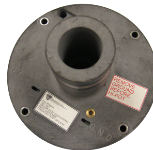
Rotor-mounted Transmitter
